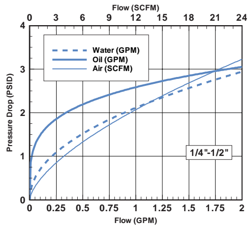
SERIES 3 -02 FLOW METER
